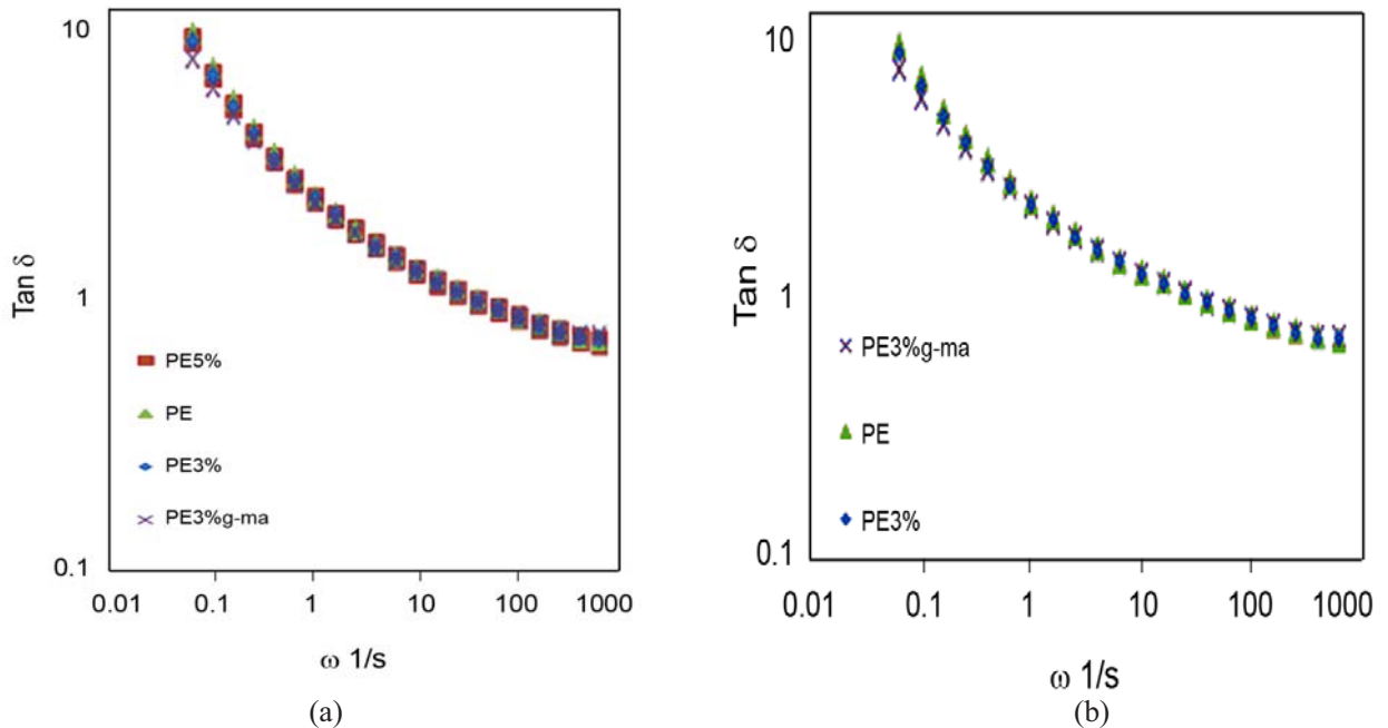
Figure 2: Tan \delta of PE/ nano-ZnO composites prepared with different concentration of nanoparticles and (b) PE With composites concentration PE/ 3% ZnO and PE/ nano-ZnO concentration 3% ZnO graft maleic prepared.
