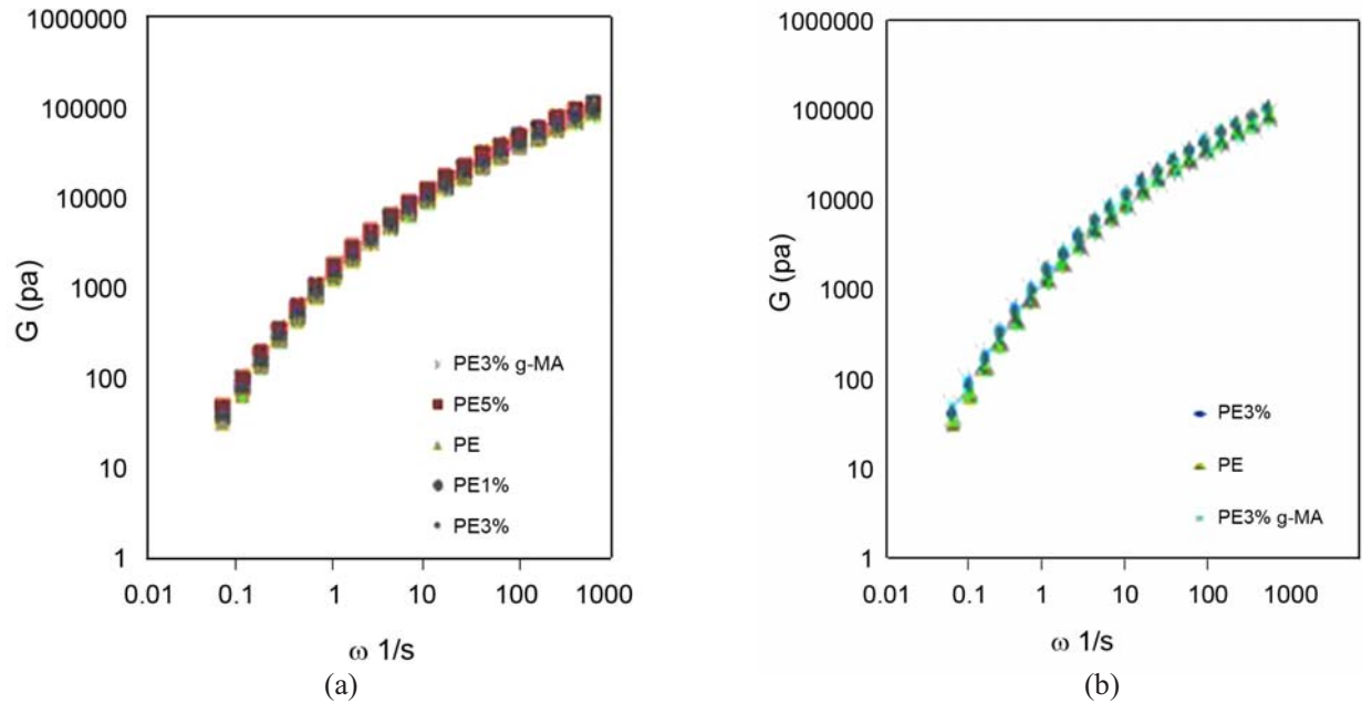
Figure 1: Dynamic modulus, (a) of PE/ nano-ZnO composites prepared with different concentration of nanoparticles and (b) PE With composites concentration PE/ 3% ZnO and PE/ nano-ZnO concentration 3% ZnO and Maleic anhydride grafted polyethylene prepared.
