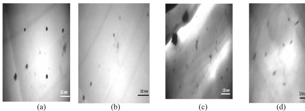
Figure 4: TEM micrograph of antimicrobial nanocomposites LDPE film a: LDPE 1% ZnO, b: LDPE 3% ZnO, c: LDPE 3% ZnO and PE g-MA, d: LDPE 5% ZnO.
