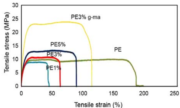
Figure 3: Tensile stress–strain curves of different ZnO LDPE films.
