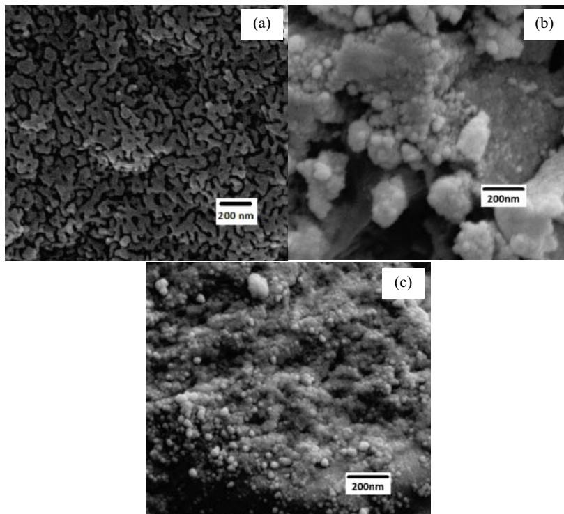
Figure 2: SEM images of the \text{TiO}_2 nanoparticles (a) as-prepared (b) annealed at 600^\circ\text{C} in presence of nitric acid (c) annealed at 600^\circ\text{C} in absence of nitric acid.
