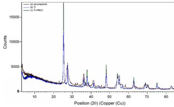
Figure 1: XRD pattern of \text{TiO}_2 nanoparticles (a) as-prepared (red line) (b) annealed at 600^\circ\text{C} without nitric acid (blue line) (c) annealed at 600^\circ\text{C} with nitric acid (green line).
