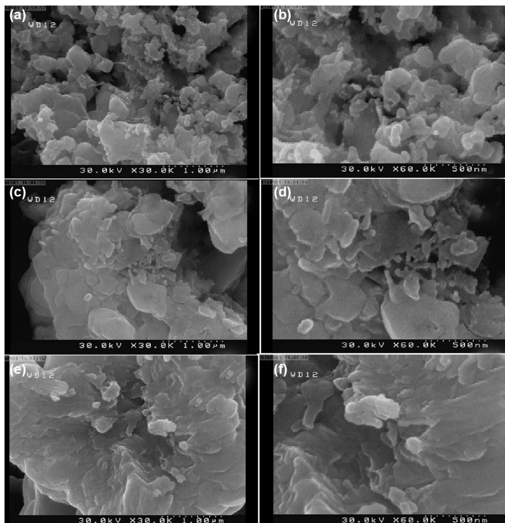
Figure 3: FE-SEM photographs of CuO nanoparticles synthesized using 20 mL (a,b), 40 mL (c,d) and 80 mL (e,f) of sour cherr juice.
