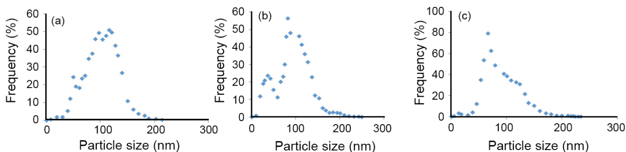
Figure 4: Diagram of CuO particles size synthesized using (a) 20 mL, (b) 40 mL, and (c) 80 mL of sour cherry juice.
