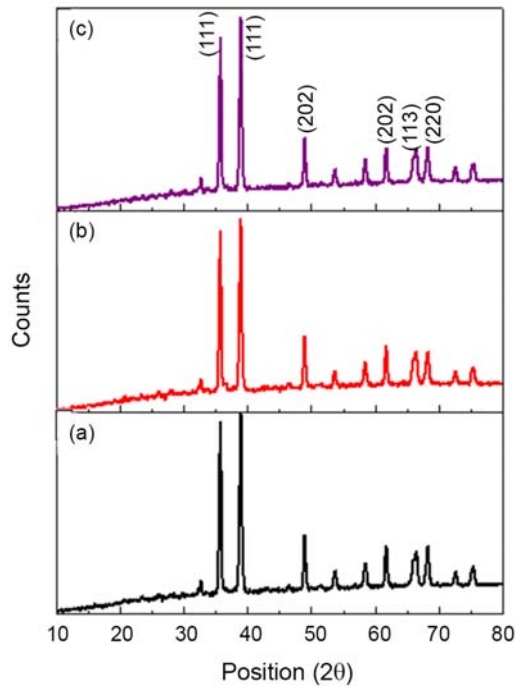
Figure 1: XRD patterns of CuO particles synthesized using (a) 20 mL; (b) 40 mL (c) 80 mL of Sour Cherry juice.
