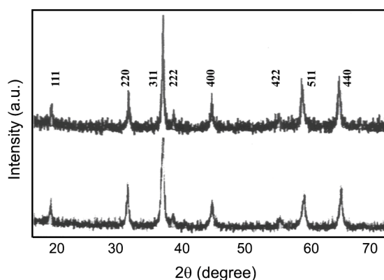
Fig. 2: XRD patterns of the \text{Co}_3\text{O}_4 nanoparticles prepared from a) 1 and b) 2.
