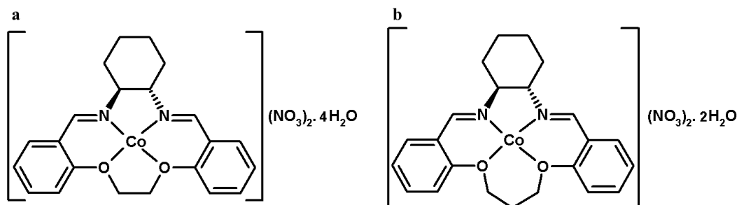
Scheme 1: The chemical structures of a) (1) and b) (2).
