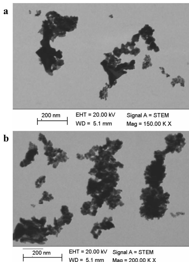
Fig. 3: TEM images of the \text{Co}_3\text{O}_4 nanoparticles prepared from a) 1 and b) 2.
