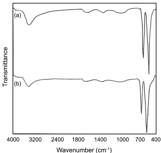
Fig. 1: FT-IR spectra of the \text{Co}_3\text{O}_4 nanoparticles prepared from a) (1) and b) (2).
