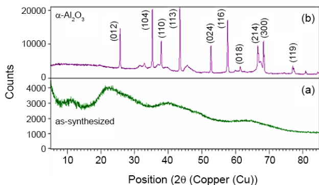
Fig. 1. XRD pattern of \text{Al}_2\text{O}_3 nanocrystals, (a) as-synthesized and (b) annealed at 1000^\circ\text{C}
