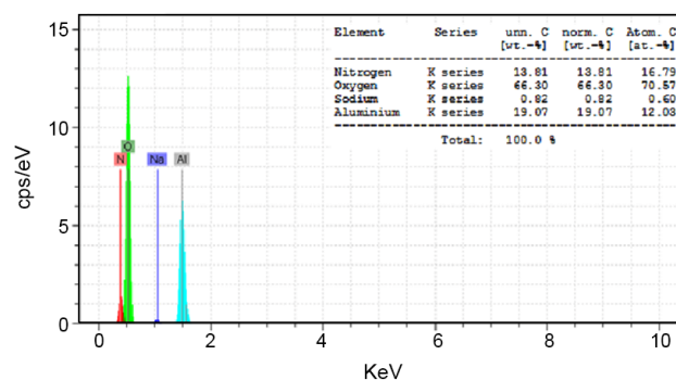
Fig. 4. EDS spectra of the as-synthesized \text{Al}_2\text{O}_3 .
