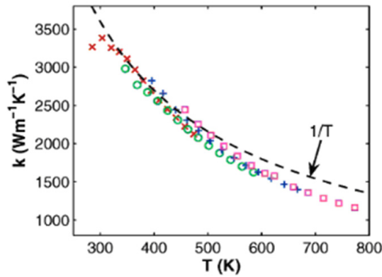
Fig. 4: Thermal conductivity of SWCNT in the temperature range 300-800K.
