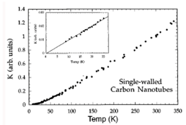
Fig. 1: Thermal conductivity of SWNT as a function of temperature.
