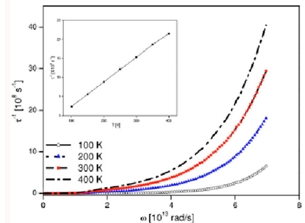
Fig. 2: Relaxation rates of Umklapp process of (6, 0) SW-CNT.
