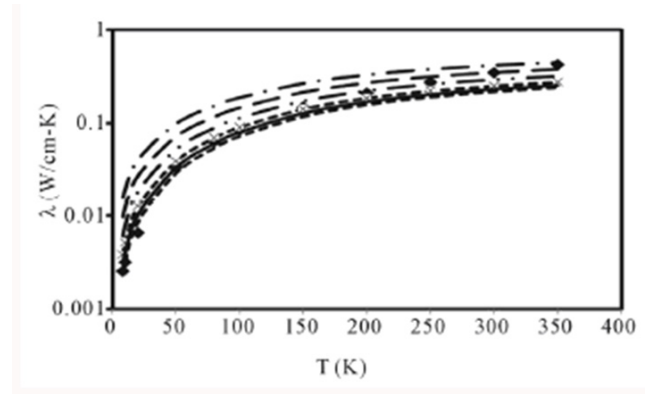
Fig. 3: Thermal conductivity of SWCNT in the temperature range 8-350 at different diameters (0.7, 0.75, 0.8, 0.9, 1, and 1.1).
