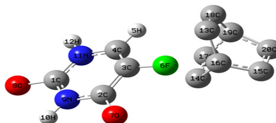
Fig. 6. Optimized structure of 5-Fluorouracil and Carbon nanocone: P2
