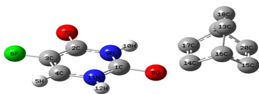
Fig. 5. Optimized structure of 5-Fluorouracil and Carbon nanocone: P1
