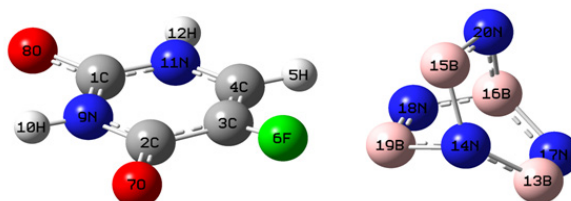
Fig. 9. Optimized structure of 5-Fluorouracil and BN nanocone: P2
