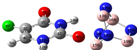
Fig. 8. Optimized structure of 5-Fluorouracil and BN nanocone: P1
