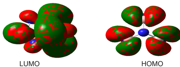
Fig. 7. HOMO and LUMO orbitals of BN nanocone
