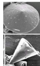
Fig. 2. Carbon nanocone from three view
