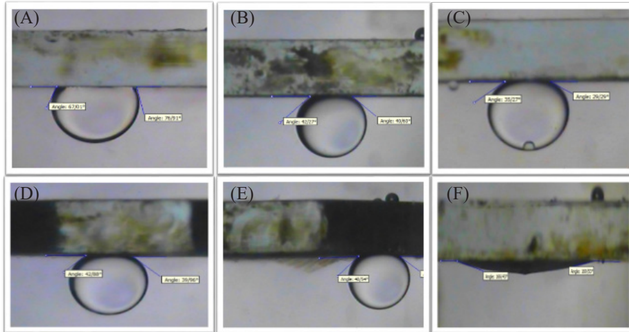
Fig. 6. A - low salinity and 0.1 wt% nano-silica , B - low salinity and 0.5 wt% nano-silica , C - low salinity and 0.75 wt% nano-silica, D - low salinity and 1 wt% nano-silica , E - low salinity and nano-silica in the end, F - low salinity and 2 wt% nano-silica
