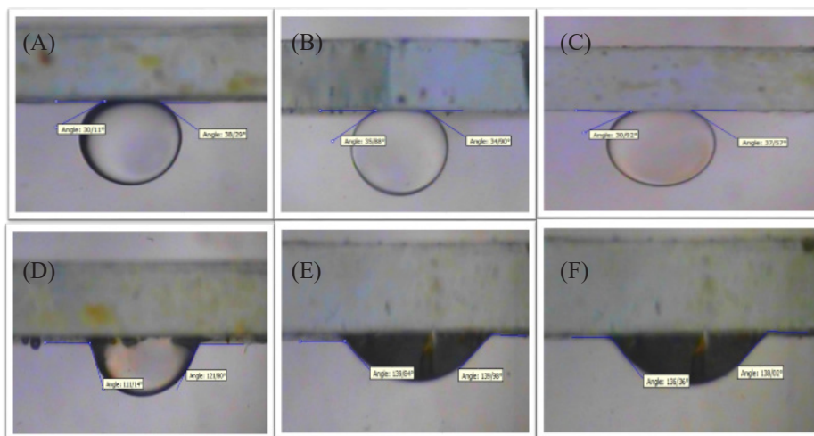
Fig. 5. A - 0.01% salinity at 80 degree temperature , B - 0.05% salinity at 80 degree temperature , C - 0.1% salinity at 80 degree temperature , D - 0.2% salinity at 80 degree temperature , E - 0.2% salinity at 80 degree temperature , F - 1% salinity at 80 degree temperature
