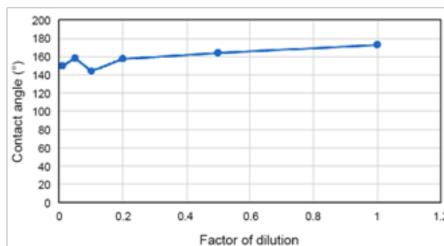
Diagram 2. Examining the effect of seawater diluting on wettability change of oil-wet silica surface
