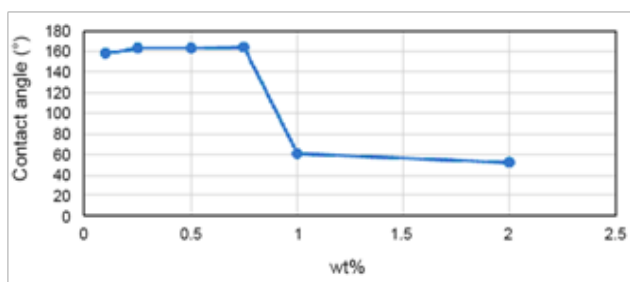
Diagram 1. Examining the effect of different concentrations of silica nanoparticles on silica surfaces wettability
