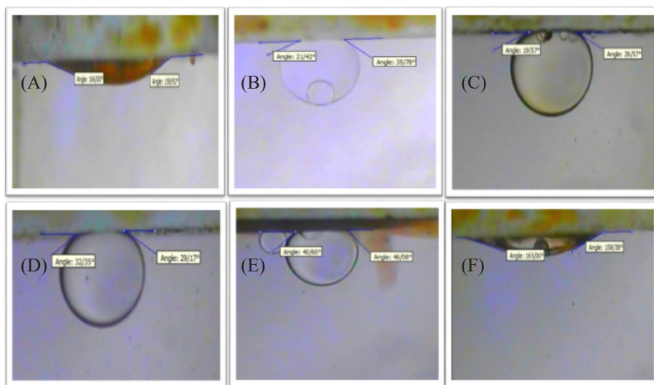
Fig. 7. A - 0.01% salt water and 0.25 wt% nano silica , B - 0.05% salt water and 0.25 wt% nano silica , C - 0.1% salt water and 0.25 wt% nano silica , D- 0.2% and 0.25 wt% of salt water and nano-silica , E 1% salt water and 0.25 wt% of nano-silica , F salt water, 0.5 and 0.25 wt% of nano-silica
