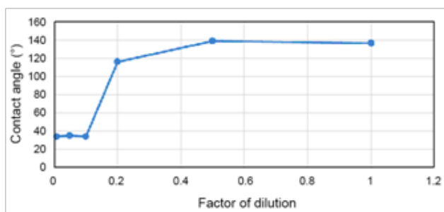
Diagram 3. Examining the effect of seawater diluting on wettability change of oil-wet silica surface in 80 degree centigrade temperature
