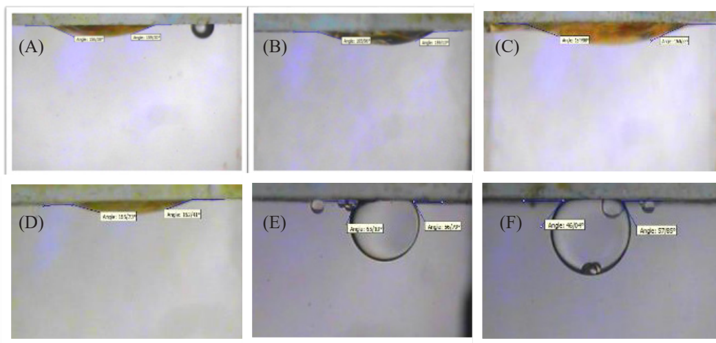
Fig. 3. A - 0.1 wt% of nano-silica , B - 0.25 wt% of nano-silica , C - 0.5 wt% of nano-silica , D - 0.75 wt% of nano-silica, E - 1 wt% of nano-silica , F - 2 wt% of nano-silica
