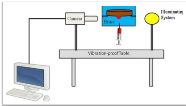
Fig. 1. Schematic measurement of contact angle by sessile drop method
