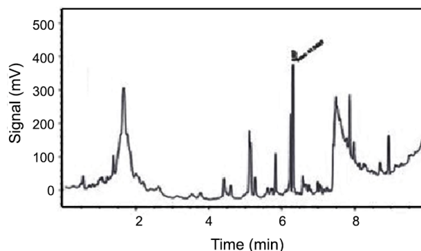
Fig. 1. Standard chromatogram.
