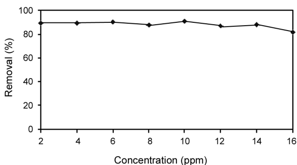
Figure 4: Effect of CNB concentrations on adsorption of it onto MWCNTs. [MWCNTs]_0=0.1 g/250mL, [pH]_0=5.4 ; Contact Time=60 min.
