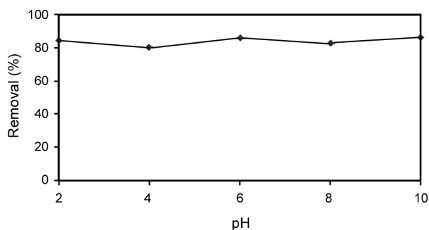
Figure 2: Effect of pH on adsorption of CNB onto MWCNTs. [CNB]_0=16 mg/L; [MWCNTs]_0=0.1 g/250mL; Contact Time=60 min.
