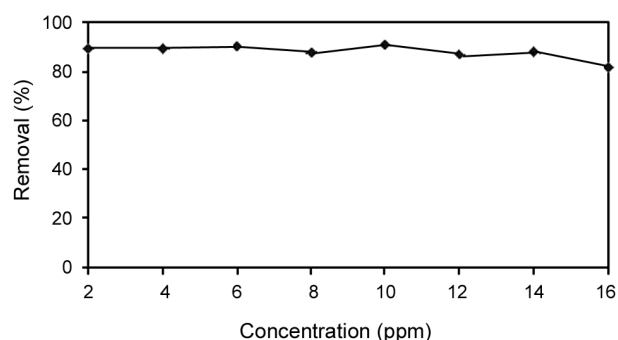
Figure 3: Effect of MWCNTs dosage on adsorption of CNB onto MWCNTs. [CNB]_0=16 mg/L; [pH]_0=5.4 ; Contact Time=60 min.
