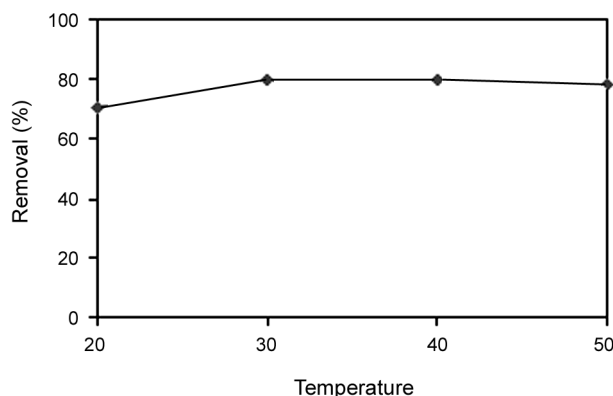
Figure 5: Effect of temperature on adsorption of CNB onto MWCNTs. [CNB]_0=16 mg/L; [MWCNTs]_0=0.1 g/250mL, [pH]_0=5.4 ; Contact Time=60 min.
