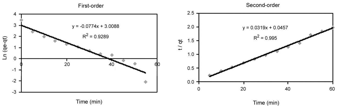
Figure 7: First and second order kinetics for the adsorption of CNB onto MWCNTs.
