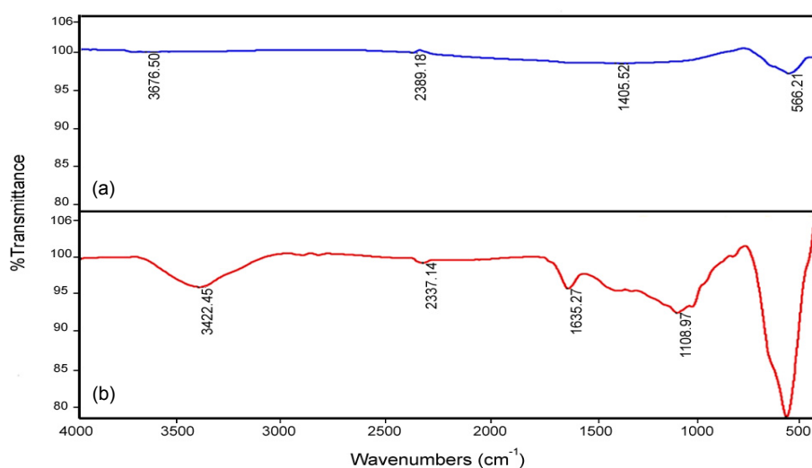
Figure 4: FTIR spectrum of \text{CoFe}_2\text{O}_4 nanoparticles (a) without and (b) with calcination.
