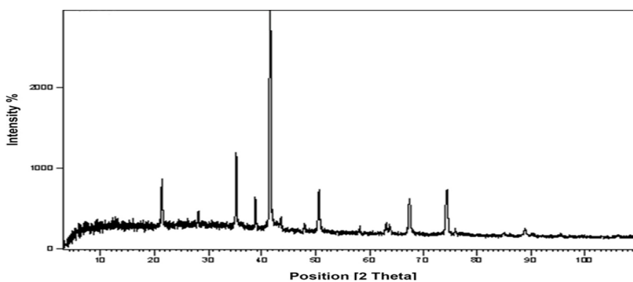
Figure 2: X-ray diffraction pattern of \text{CoFe}_2\text{O}_4 synthesis in present of GMO as a surfactant.
