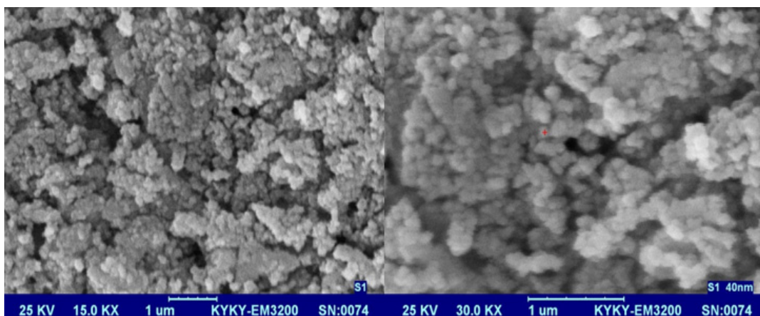
Figure 3: SEM imaging of \text{CoFe}_2\text{O}_4 nanoparticles synthesized with GMO as surfactant.
