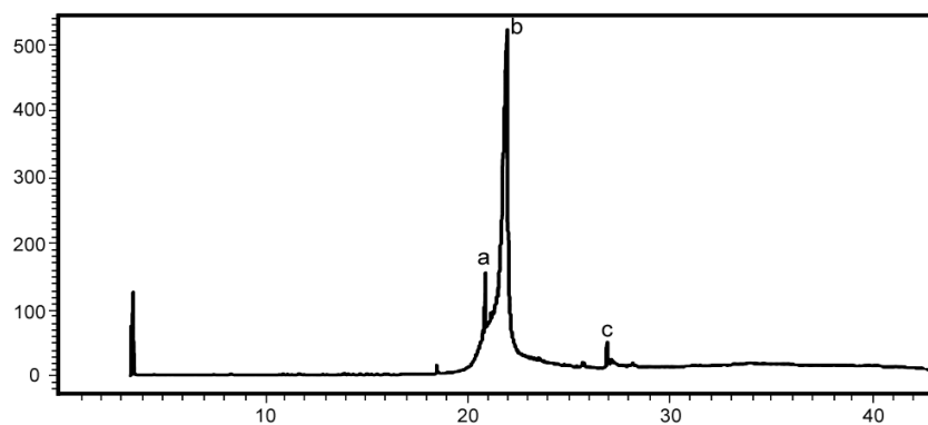
Figure 1: GC spectrum of products a) glycerol monooleat, b) β-glycerol monooleat and c) glycerol dioleat.
