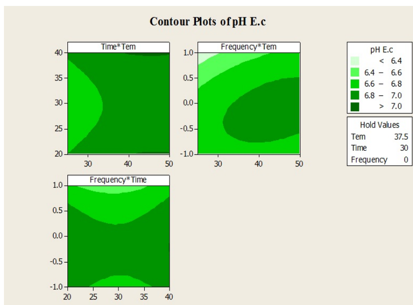
Figure 2-A: Effects of time, temperature and frequency of ultrasound on pH.
