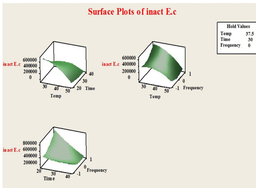
Figure 1-B: Surface plots of effects of time temperature and frequency of ultrasound on E. coli inactivation.
