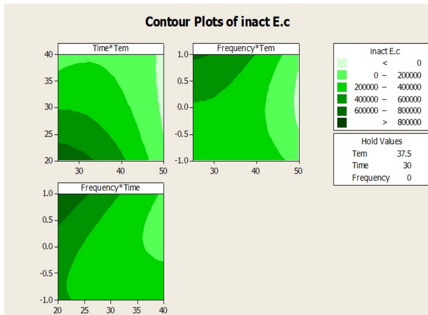
Figure 1-A: Effects of temperature and frequency of ultrasound on E. coli inactivation.
