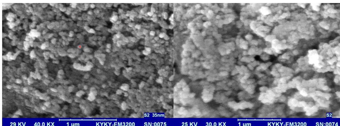
Figure 2: SEM imaging of \text{CoFe}_2\text{O}_4 nano-particles synthesized with OA as a surfactant.
