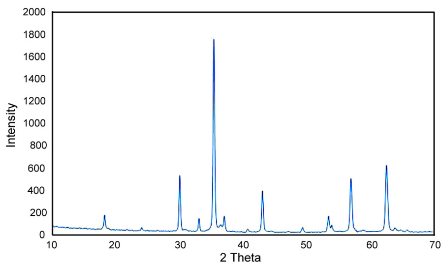
Figure 1: X-ray diffraction pattern of \text{CoFe}_2\text{O}_4 synthesis in the presence of OA as a surfactant.
