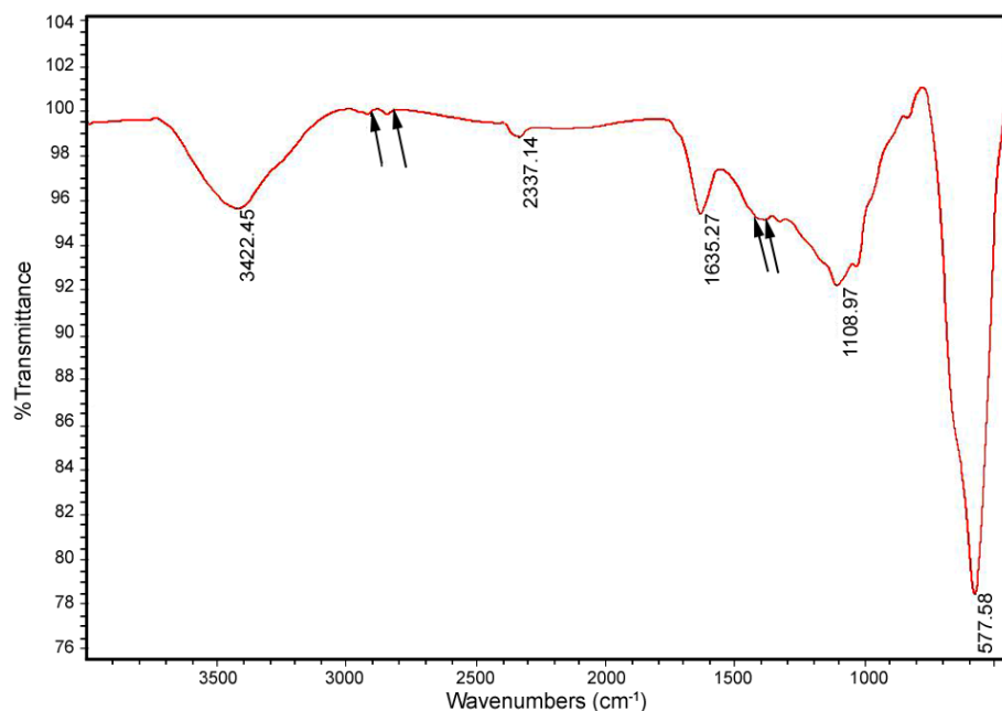
Figure 3: FTIR spectrum of un-calcined \text{CoFe}_2\text{O}_4 nano-particles.
