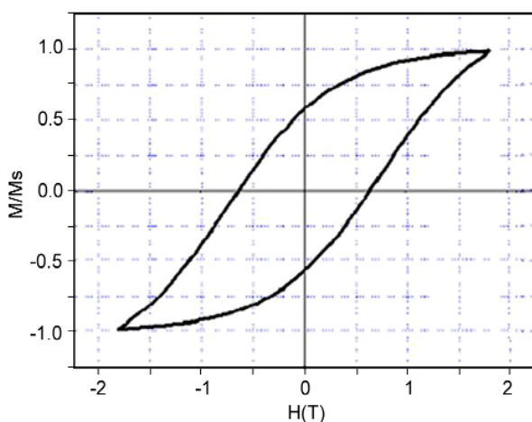
Figure 5: Magnetic hysteresis loops of annealed FePt nanoparticle.
