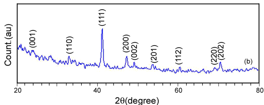
Figure 4: XRD patterns of the annealed FePt nanoparticles.
