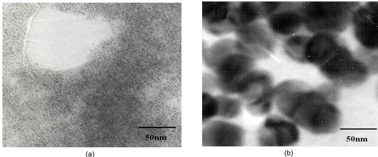
Figure 2: TEM image of the (a) as-synthesis and (b) annealed FePt nanoparticles.
