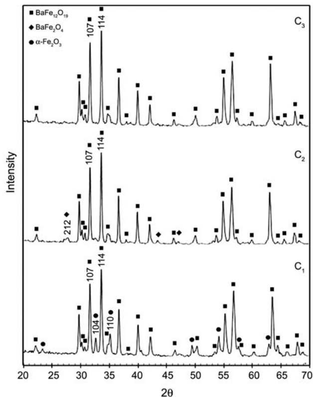
Figure 1: X-ray diffraction pattern of BaFe_{12}O_{19} synthesis in different pH.
